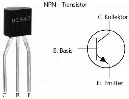
NPN - Transistor
